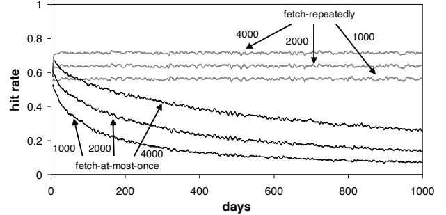
Figure 8: File-sharing effectiveness diminishes with client age. After an initial cache warm-up period, the request stream generated by fetch-at-most-once client behavior experiences rapidly decreasing cache performance, while the stream generated by fetch-repeatedly clients remains stable. This effect is shown for various cache sizes (1000, 2000, and 4000 objects).
